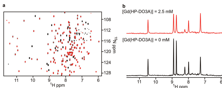
Figure 1. ^1\text{H} – ^{15}\text{N} TROSY spectra of free hUNG and the effect of the Gd(HP-DO3A) paramagnetic cosolute. (a) The spectra were obtained with ^2\text{H} , ^{15}\text{N} -enriched hUNG samples with no Gd(HP-DO3A) (black) or [\text{Gd}(\text{HP-DO3A})] = 2.5 \text{ mM} (red). (b) Representative 1D slices ( f_1 = 123.8 \text{ ppm} ) of the spectra in (a).
