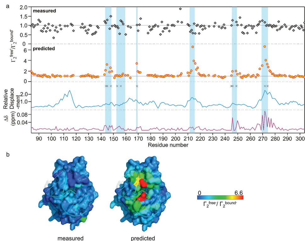
Figure 4. Measured and predicted ratios of \Gamma_2^{\text{free}}/\Gamma_2^{\text{bound}} across the hUNG linear sequence and comparison with dynamic properties, DNA-induced chemical shift changes, and relative backbone amide nitrogen atom displacements obtained in a course-grain normal-mode analysis. (a) From top to bottom: measured and predicted ratios of \Gamma_2^{\text{free}}/\Gamma_2^{\text{bound}} , amide nitrogen displacements in the lowest frequency normal-mode analysis of free hUNG (1AKZ), and weighted chemical shift ( ^1\text{H} and ^{15}\text{N} ) perturbations brought about by DNA binding. The black asterisks indicate amide positions with k_{\text{ex}} values in millisecond range. 16 Vertical blue shaded bars indicate the six regions of the primary sequence that are important for DNA binding or enzyme catalytic activity. Table S1 lists all of the PREs, chemical shift perturbations, relative atom displacements in the normal-mode analysis, and residues with chemical exchange contributions to their line widths. (b) Crystal structures of exosite hUNG–DNA complex (2OXM) with the measured (left) and predicted (right) \Gamma_2^{\text{free}}/\Gamma_2^{\text{bound}} ratios color coded to the surface.
