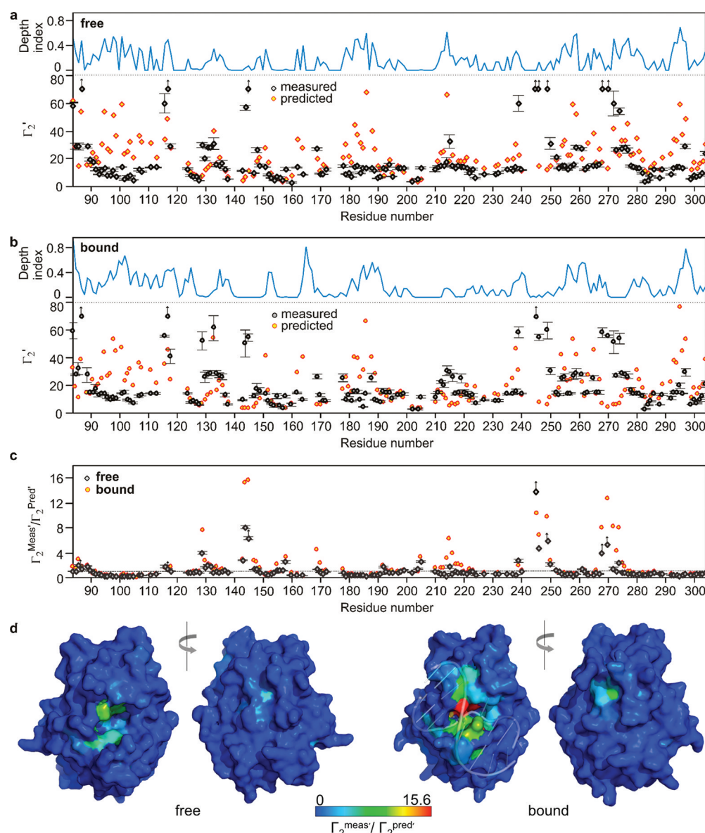
Figure 3. Measured and predicted values for the amide proton molar relaxivities ( \Gamma_2' ) of free hUNG and its complex with nontarget DNA and the calculated depth indices for each amide proton ( D_{ii} ). (a) Measured and predicted \Gamma_2' values for each amide proton of free hUNG and its corresponding depth index value (eq 2). (b) Measured and predicted \Gamma_2' values for each amide proton of DNA-bound hUNG and its corresponding depth index value (eq 2). The predicted PREs were obtained using the grid-based approach using the atom coordinates obtained from the crystal structures of the free enzyme (1AKZ) and its nonspecific DNA complex (2OXM) with water molecules omitted. 3,18,19 The predicted values were scaled to the measured PRE values using a uniform scaling factor. (c) Ratios between the measured and predicted PRE values across the protein sequence for free hUNG and its complex with DNA. (d) Crystal structures of free hUNG and its exosite hUNG–DNA complex with the ratios of \Gamma_2^{\text{meas}}/\Gamma_2^{\text{pred}} color coded to the structural surfaces. In panels a, b, and c, the missing points are either due to proline residues or residues with no or very weak signals. Errors of the data from the hUNG–DNA complex were omitted for clarity but are similar to those shown for the free enzyme. Table S1 lists all of the PREs and their error values.
