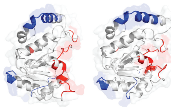
Figure 5. Two extrema of a course-grain normal-mode analysis performed using the crystallographic coordinates of free hUNG (1AKZ). Sites that are hyper-reactive and protected from the paramagnetic probe are colored in red and blue, respectively. The left panel shows the open state, and the right panel shows the closed conformation.
